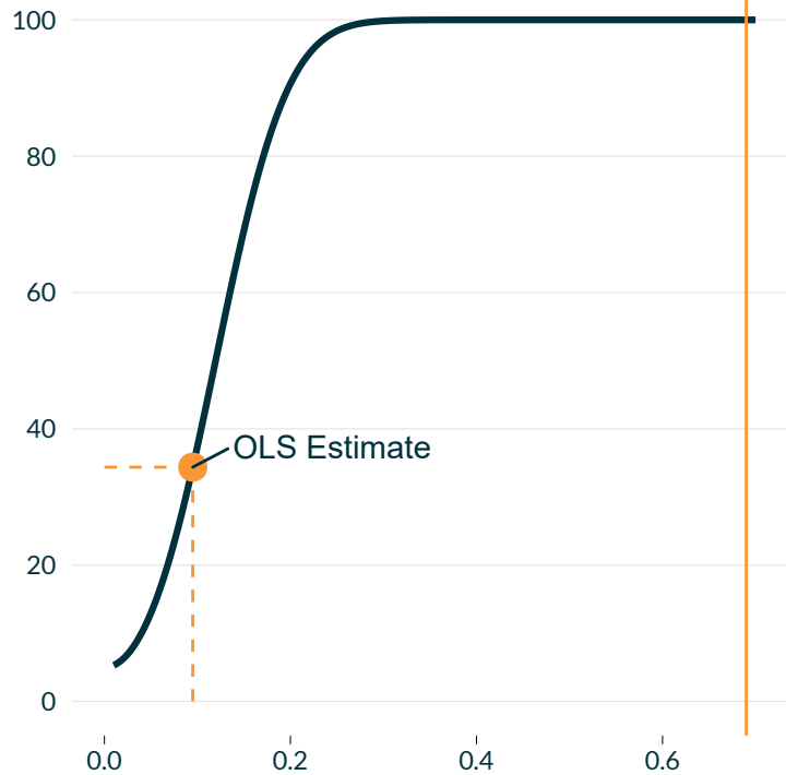
Statistical Power (%)
