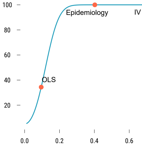
Statistical Power (%)
