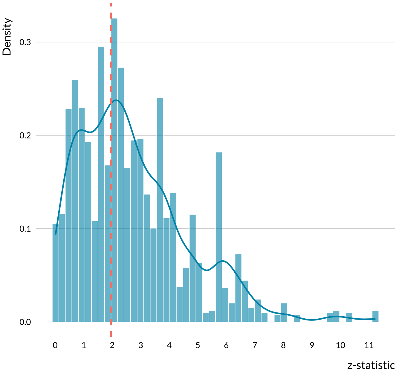
Weighted Distribution of the z-statistics More mass around the 1.96 threshold
