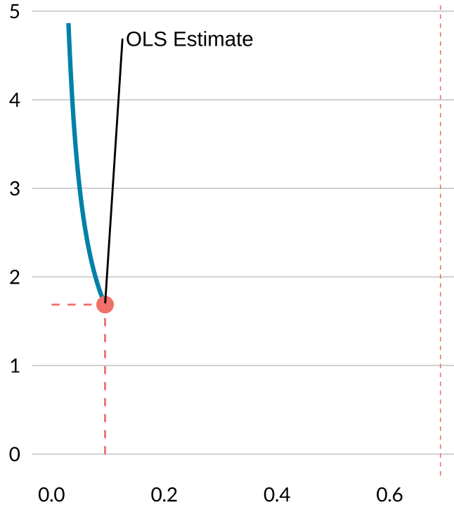
Type-M Error (Exaggeration Ratio)
