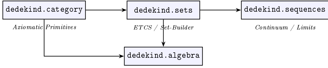
Figure 1: Module build dependencies in the dedekind library.
