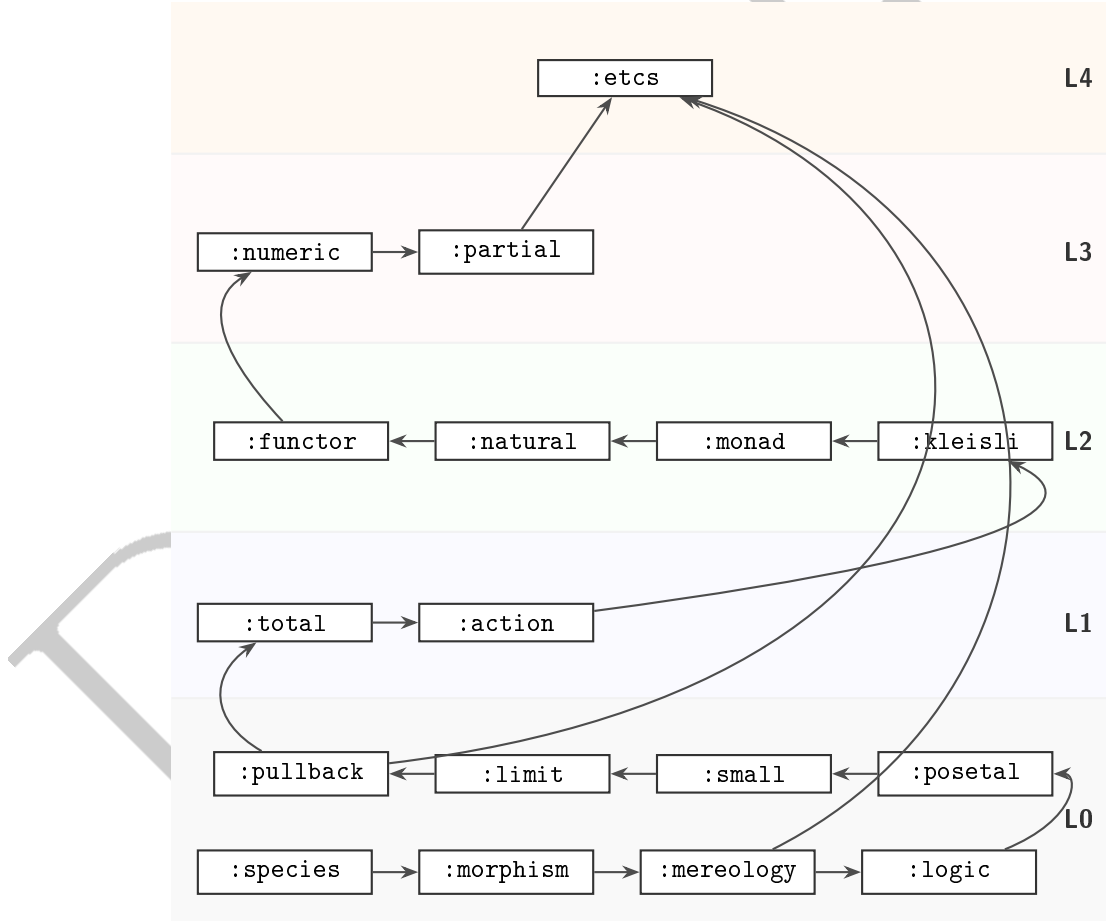
Figure 2: Refined Build Graph: The "Numeric" layer now serves as the base for "Partial" logic, allowing "ETCS" to remain decoupled from hardware specificities.
