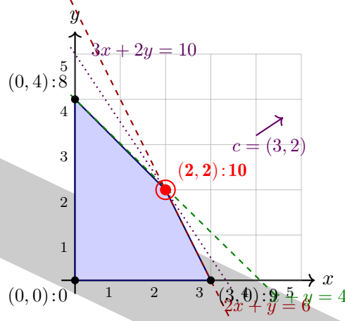
Figure 3: The feasible polygon of Showcase 9. Vertices are labelled with the objective value 3x + 2y at each. The active-set enumeration considers all \binom{4}{2} = 6 pairs of constraints; four pairs produce feasible intersections, and the optimum is the one vertex (red) where both non-axis-aligned constraints H_1: x + y \leq 4 and H_2: 2x + y \leq 6 bind simultaneously. At translation time the compiler performs this enumeration; the emitted binary contains only the literal coordinates of (2, 2) .
