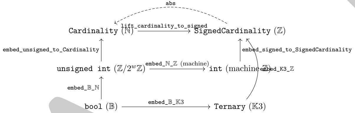
Figure 1: The carrier lattice (discrete-foundations slice). Three layers, bottom to top: truth-value carriers ( bool , Ternary ); machine integer carriers ( unsigned int = \mathbb{Z}/2^w\mathbb{Z} as a finite cyclic ring; int = machine \mathbb{Z} with UB-on-overflow); variant carriers inhabiting the textbook Forms ( Cardinality = \mathbb{N} as the Natural Numbers Object; SignedCardinality = \mathbb{Z} as the Initial Ring / Grothendieck group of \mathbb{N} ). Each labelled arrow is the actual code identifier of a canonical embedding registered as a monic morphism in dedekind.numbers . The top-row arrow lift_cardinality_to_signed is the canonical \mathbb{N} \hookrightarrow \mathbb{Z} embedding at the variant carrier layer (the Grothendieck-construction unit); the binary closure-forcing operator Cardinality – Cardinality \rightarrow SignedCardinality realises the Grothendieck construction on operator pairs and is not shown on the diagram (it would require a product node). The middle-row arrow embed_N_Z is the machine-layer sign reinterpretation static_cast<int>(unsigned) despite its variant-evocative name — the actual canonical \mathbb{N} \rightarrow \mathbb{Z} on the carriers happens at the variant layer. The dashed retraction abs is the split-mono partner of the embedding ( abs \circ embed = id on the non-negative fragment). embed_K3_Z skips the machine-int row and lands directly on SignedCardinality (a deliberate factorisation choice). Multiple paths between extremes commute up to canonical isomorphism.
