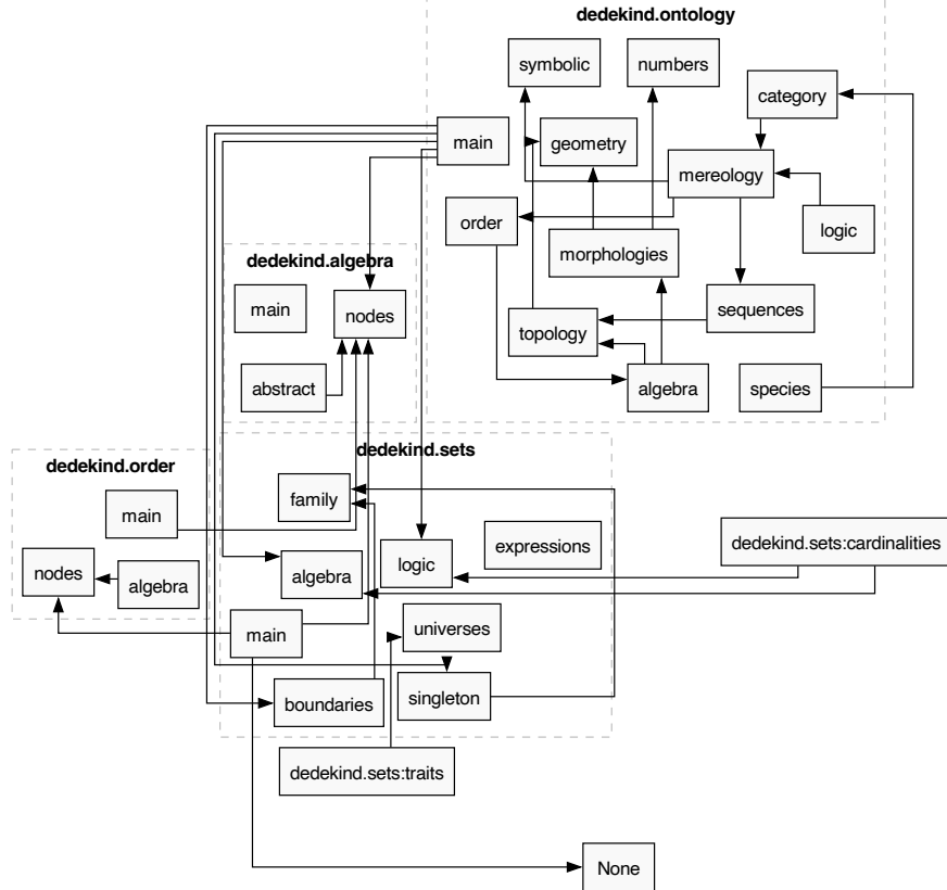
Figure 1: The Ontological Build Graph: Automated dependency resolution.
