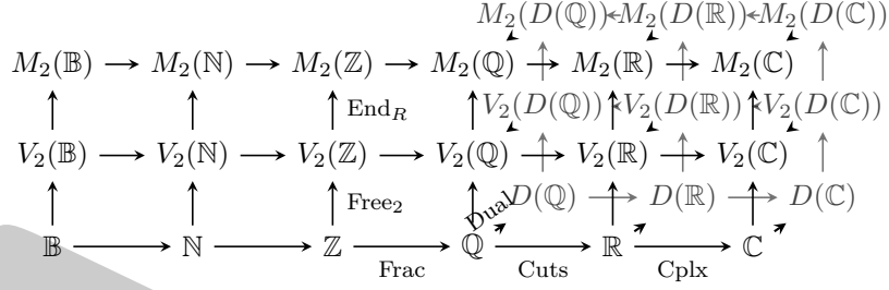
Figure 1: The Algebraic Tower (target-state Figure 1, first sketch). Two-axis lattice: horizontal = carrier-strength ( \mathbb{B} \rightarrow \mathbb{N} \rightarrow \mathbb{Z} \rightarrow \mathbb{Q} \rightarrow \mathbb{R} \rightarrow \mathbb{C} , each step a labelled functor application \text{FRAC} / \text{CUTS} / \text{CPLX} ); vertical = object rank (Scalars \rightarrow Vectors V_2(R) via \text{Free}_2 \rightarrow Matrices M_2(R) via \text{End}_R ). The finite-field side branch ( \mathbb{F}_p, \mathbb{F}_{64} ) hangs off \mathbb{Z} through the same Quot functor at prime / polynomial ideals (cf. Figure 2 for the modular-arithmetic exhibit). The Extension-Functor row (Dual / Cplx as quotient rings) names the constructions used at each step. The Machine Substrate row ( bool / uint / int / double ) sits below the Honest-Rejection boundary; the dashed arrows mark the realisation crossings that embed each machine type into its variant proxy. Hooks for the off-figure dimensions : higher rank ( V_n, M_n, n > 2 ; #368), predicate-set / order-theoretic constructions (a sibling Geometric Tower , candidate Figure 1b), tensor / exterior powers, and the trait-registry pinning of every arrow as a mechanical witness (#499). The 2D projection is necessarily lossy.
