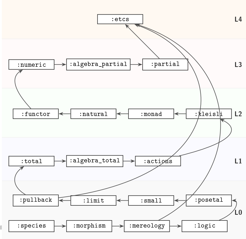
Figure 2: Refined Build Graph: The "Numeric" layer now serves as the base for "Partial" logic, allowing "ETCS" to remain decoupled from hardware specificities.
