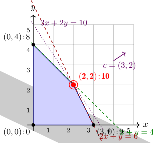
Figure 4: The feasible polygon of Showcase 9. Vertices are labelled with the objective value 3x+2y at each. The active-set enumeration considers all \binom{4}{2} = 6 pairs of constraints; four pairs produce feasible intersections, and the optimum is the one vertex (red) where both non-axis-aligned constraints H_1: x+y \leq 4 and H_2: 2x+y \leq 6 bind simultaneously. At translation time the compiler performs this enumeration; the emitted binary contains only the literal coordinates of (2, 2) .
