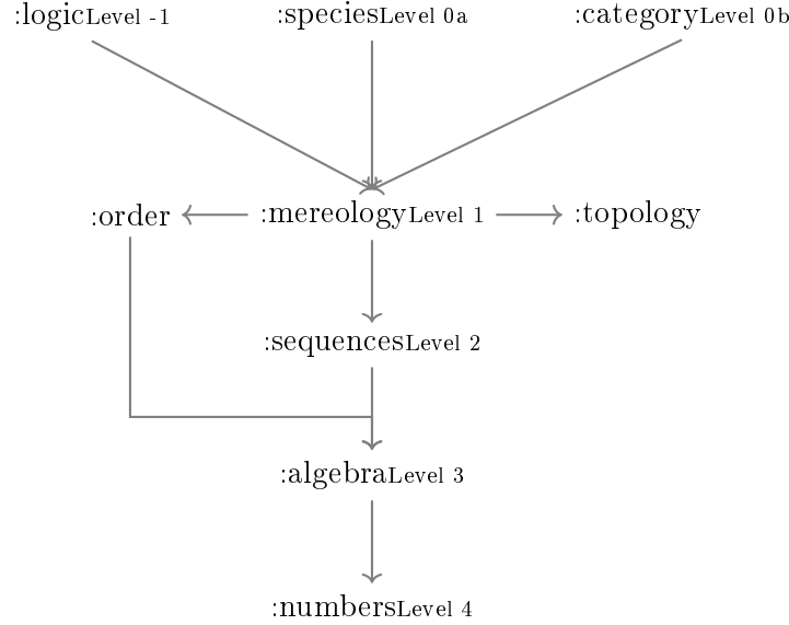
Figure 1: The Ontological Build Graph: Enforcing a Non-Circular Derivation of Truth.
