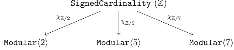
Figure 2: The universal-property reading of \mathbb{Z} as the initial ring (sibling to Figure 1). For every commutative unital ring R , the initial-object property of \mathbb{Z} supplies a unique ring homomorphism \chi_R : \mathbb{Z} \rightarrow R . The diagram exhibits this at three concrete prime targets R = \text{Modular}\langle n \rangle (the cyclic ring \mathbb{Z}/n\mathbb{Z} , with prime n \in \{2, 5, 7\} chosen so each target is a field). Each \chi_n is the mod- n reduction; the test suite [algebra][initial_ring][modular][universal-property] (in src/test/cpp/modules/dedekind/numbers/initial_ring_test.cpp ) realises \chi_n operationally as the helper χ_to_modular<n> and exercises ring-homomorphism preservation ( \chi(a + b) = \chi(a) + \chi(b) , \chi(a \cdot b) = \chi(a) \cdot \chi(b) , \chi(1_{\mathbb{Z}}) = 1_R ) plus sign-aware mod reduction. A complementary structural reading: unsigned int \cong \text{Modular}\langle 2^w \rangle at the machine layer (the carrier-lattice middle row of Figure 1 is the same diagram unrolled at the machine width); bool \cong \text{Modular}\langle 2 \rangle under XOR. The figure is the visual companion to the engineer’s honesty obligation that universal-property uniqueness imposes: declaring is_initial_ring_v<SignedCardinality> = true is the type-system anchor; the operational behaviour at every concrete target is the test-suite obligation.
