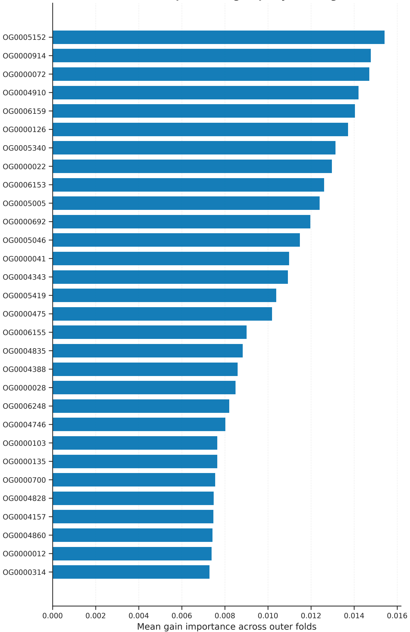
Scenario A: top 30 Orthogroups by XGBRF gain
