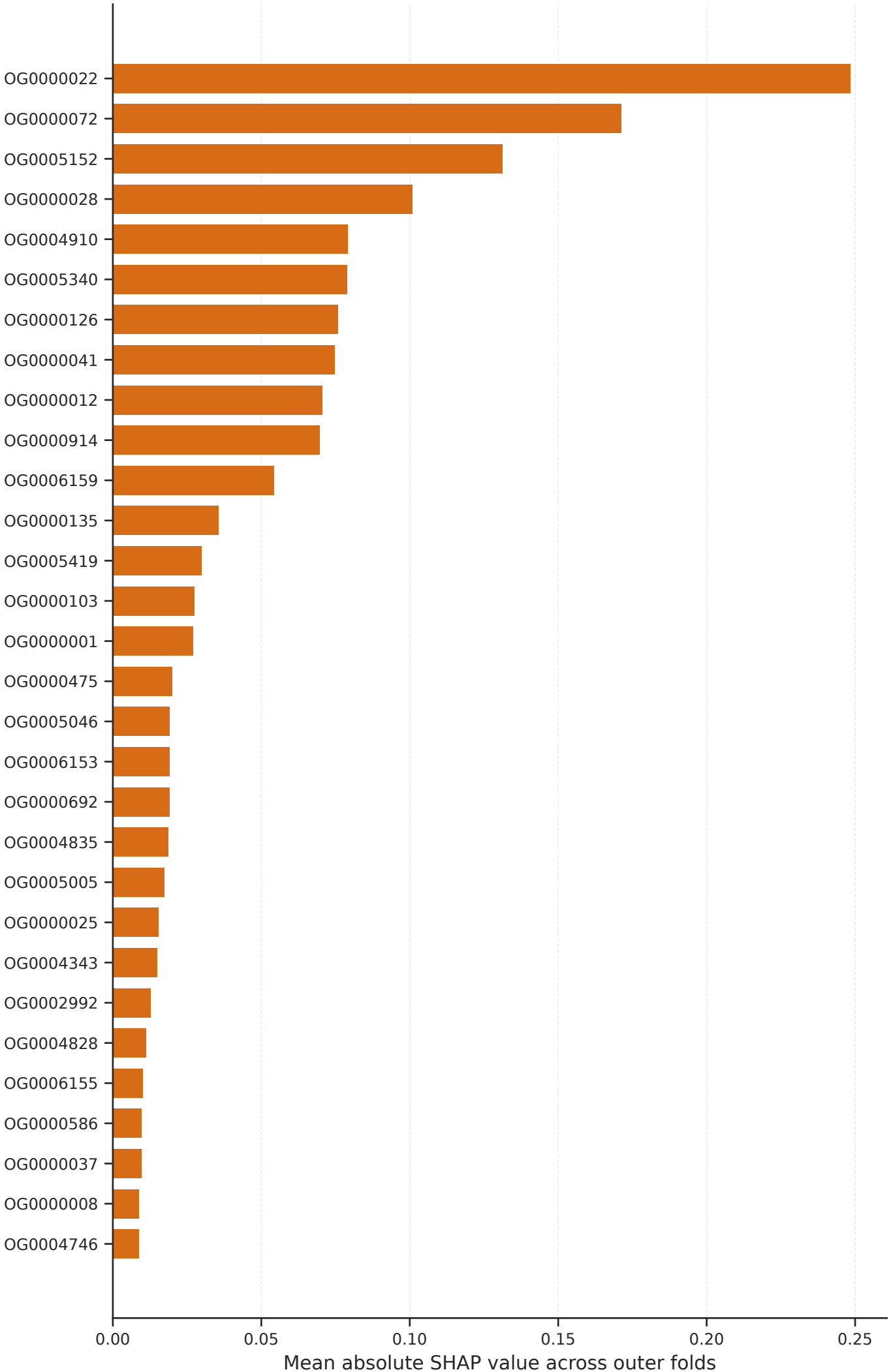
Scenario A: top 30 Orthogroups by SHAP importance
