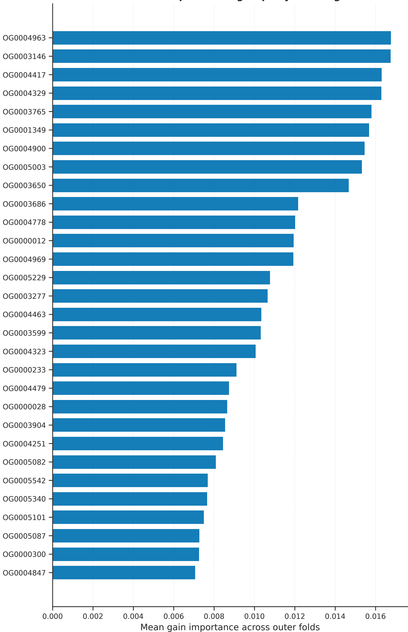
Scenario B: top 30 Orthogroups by XGBRF gain
