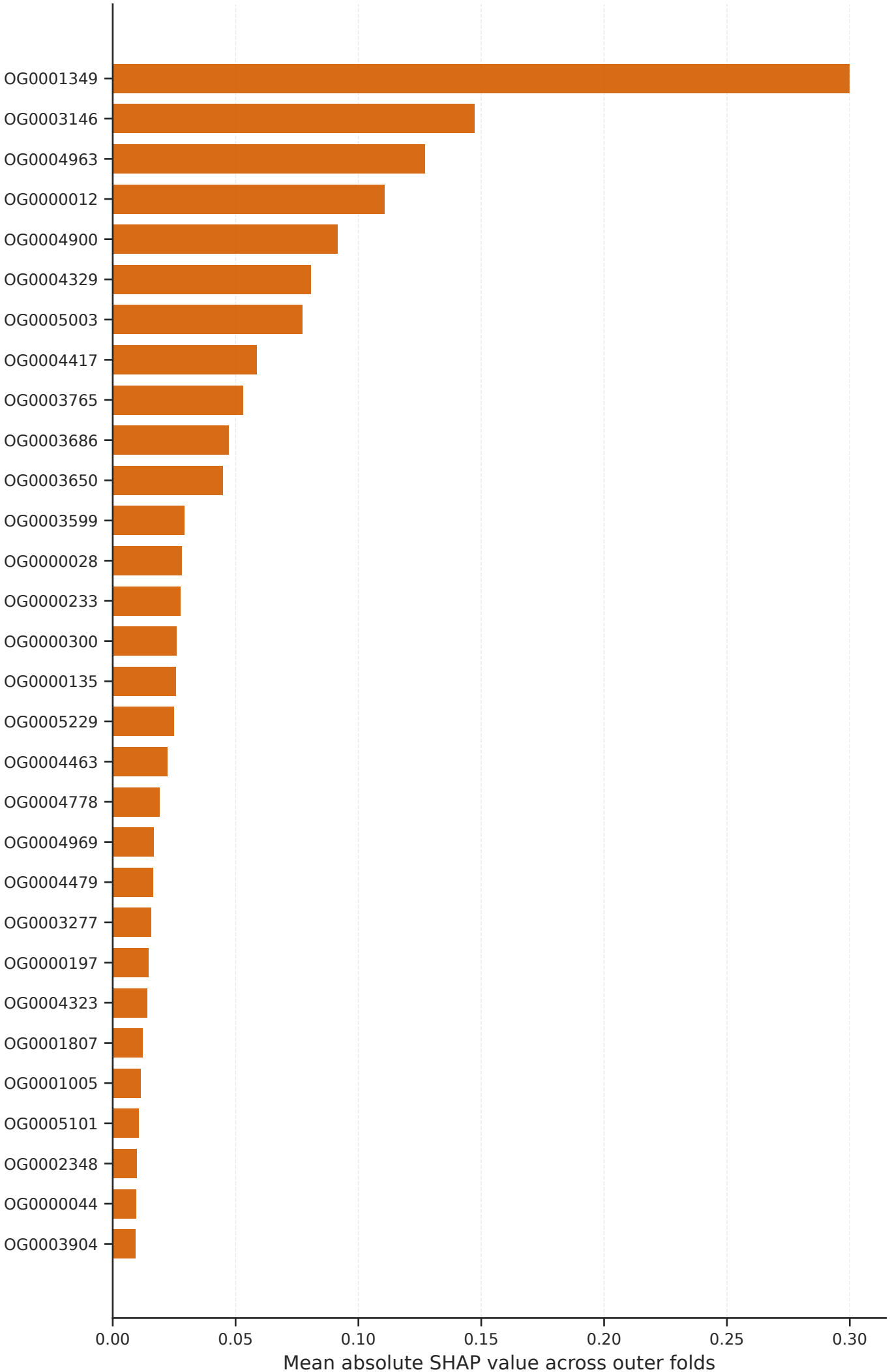
Scenario B: top 30 Orthogroups by SHAP importance
