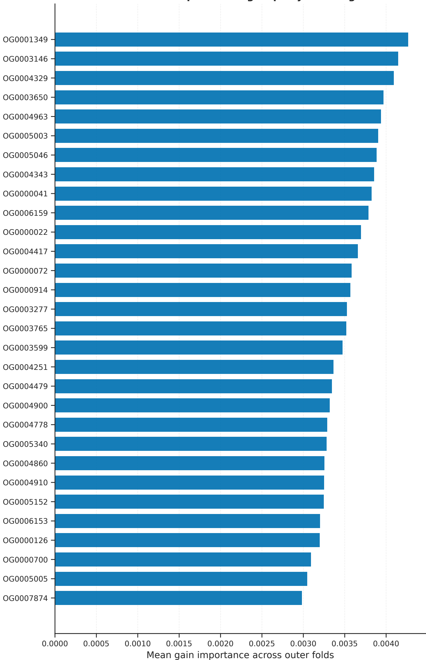
Scenario C: top 30 Orthogroups by XGBRF gain
