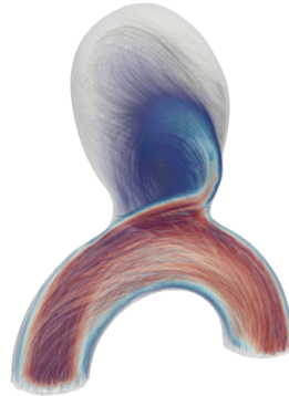
In-MGN
