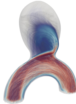
In-PI-MGN
