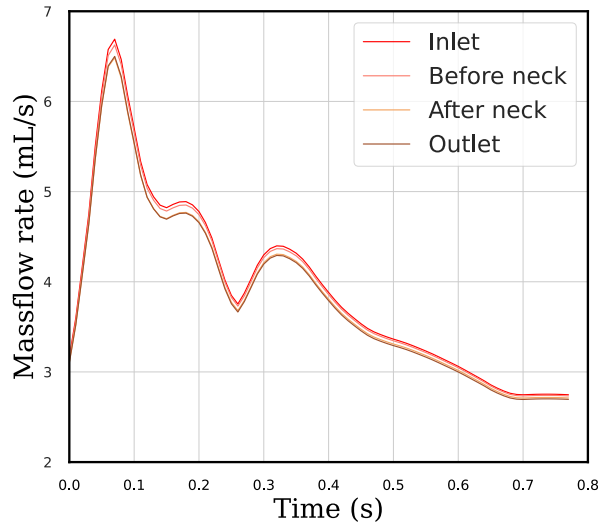
Mass flow over time from CFD ground truth
