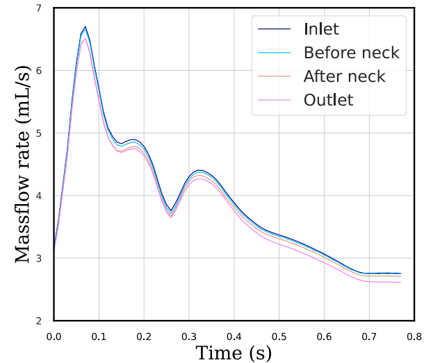
Mass flow over time from In-PI-MGN prediction
