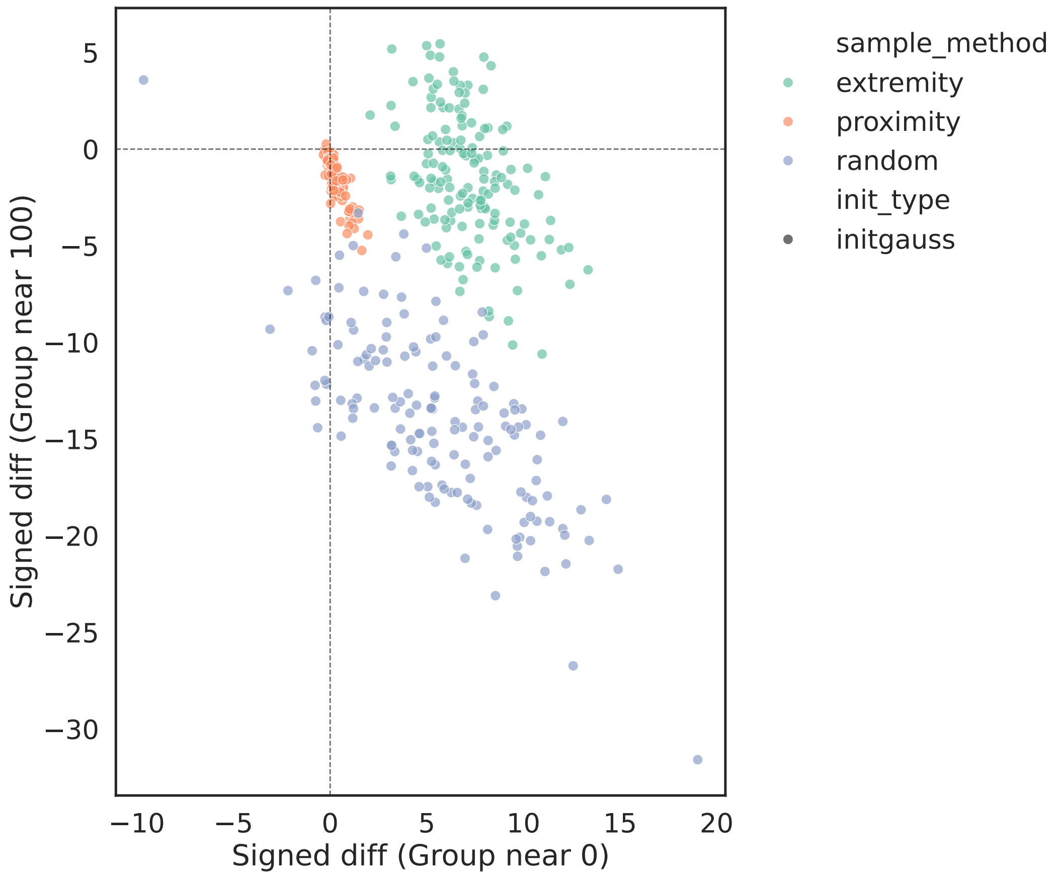
False polarization vs false moderation
