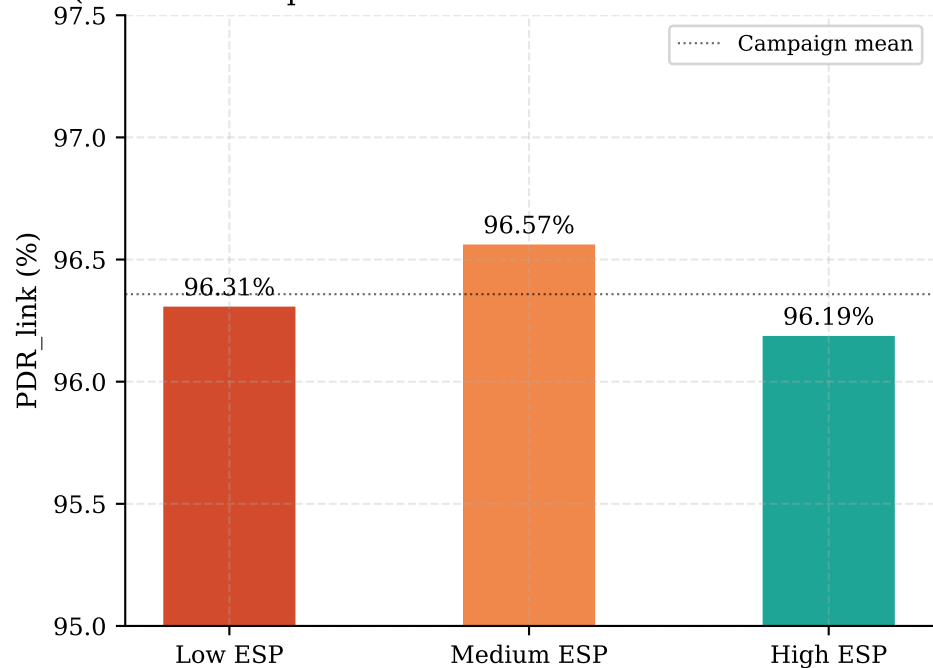
E18: ESP Tier PDR (no monotone pattern — confirms collision-dominated losses)
