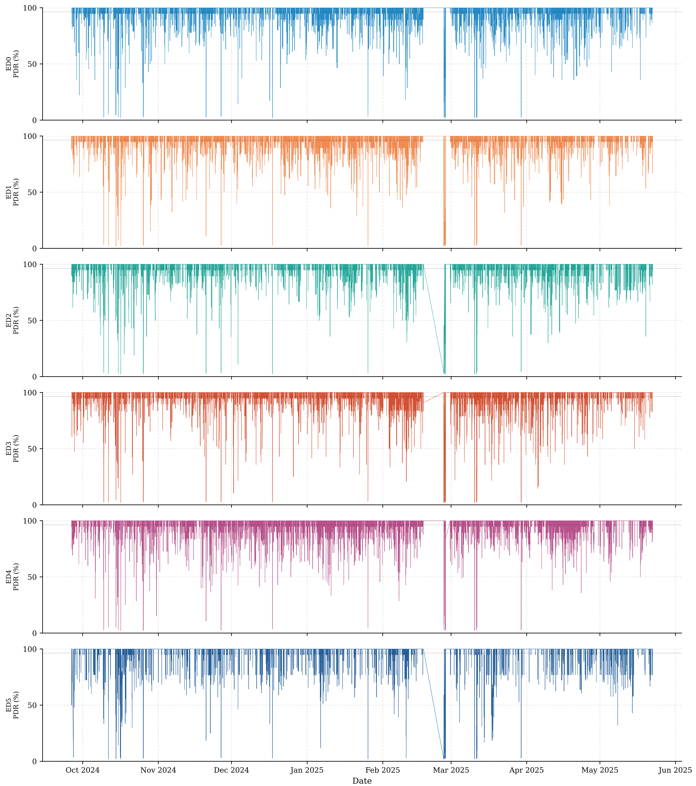
Fig 7.3 — Rolling 30-min PDR per Device (Sep 2024-May 2025) Dotted = PDR_link mean (96.36%)
