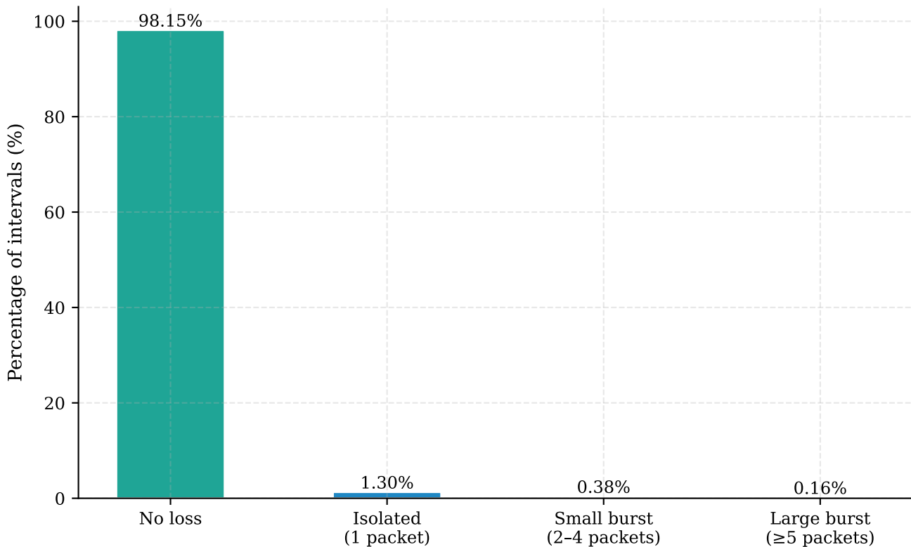
Fig 7.4 — Burst Loss Distribution (E16)
