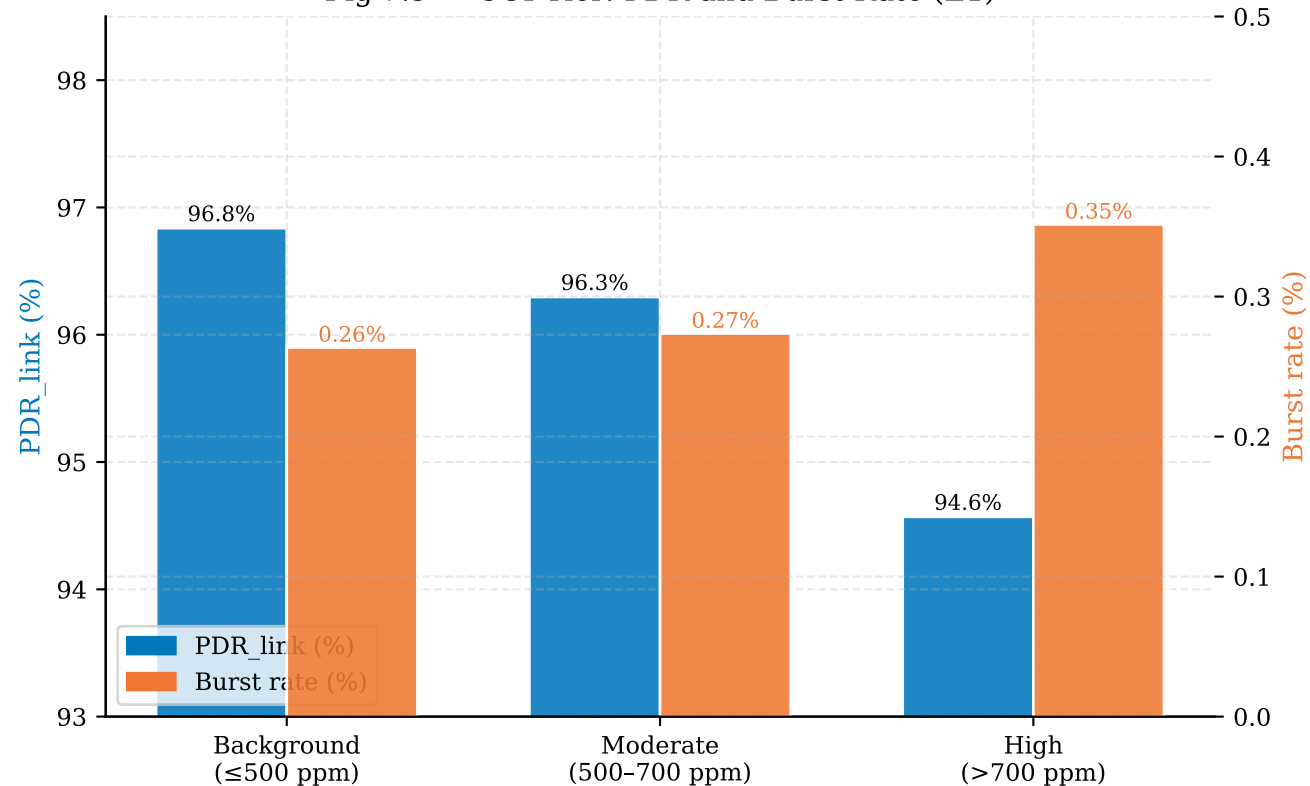
Fig 7.9 — CO 2 Tier: PDR and Burst Rate (E1)
