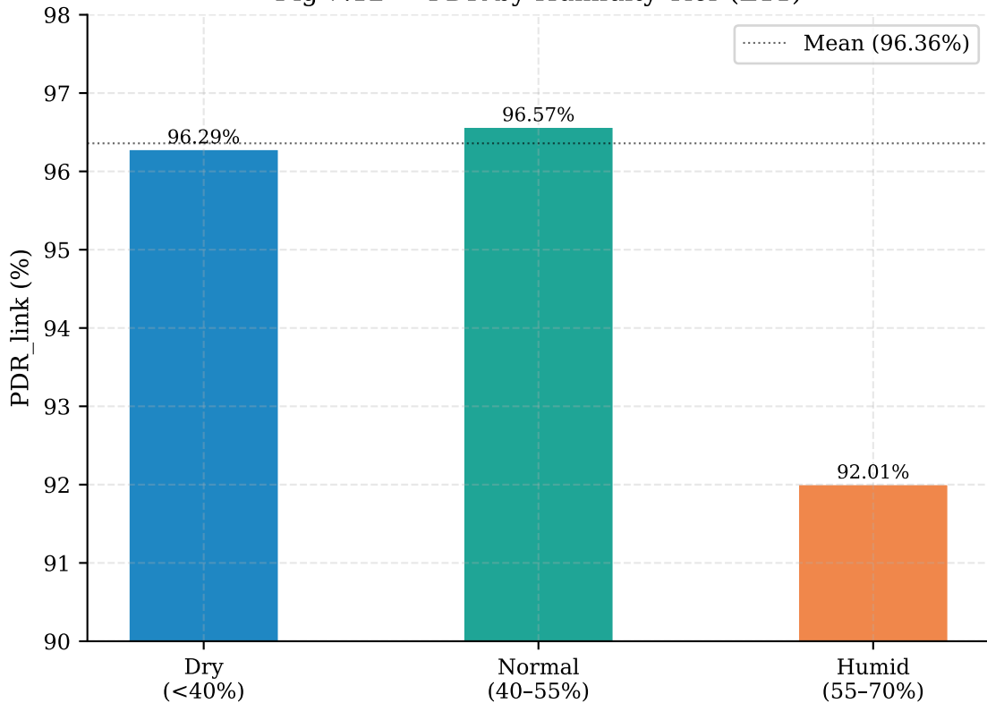
Fig 7.12 — PDR by Humidity Tier (E11)
