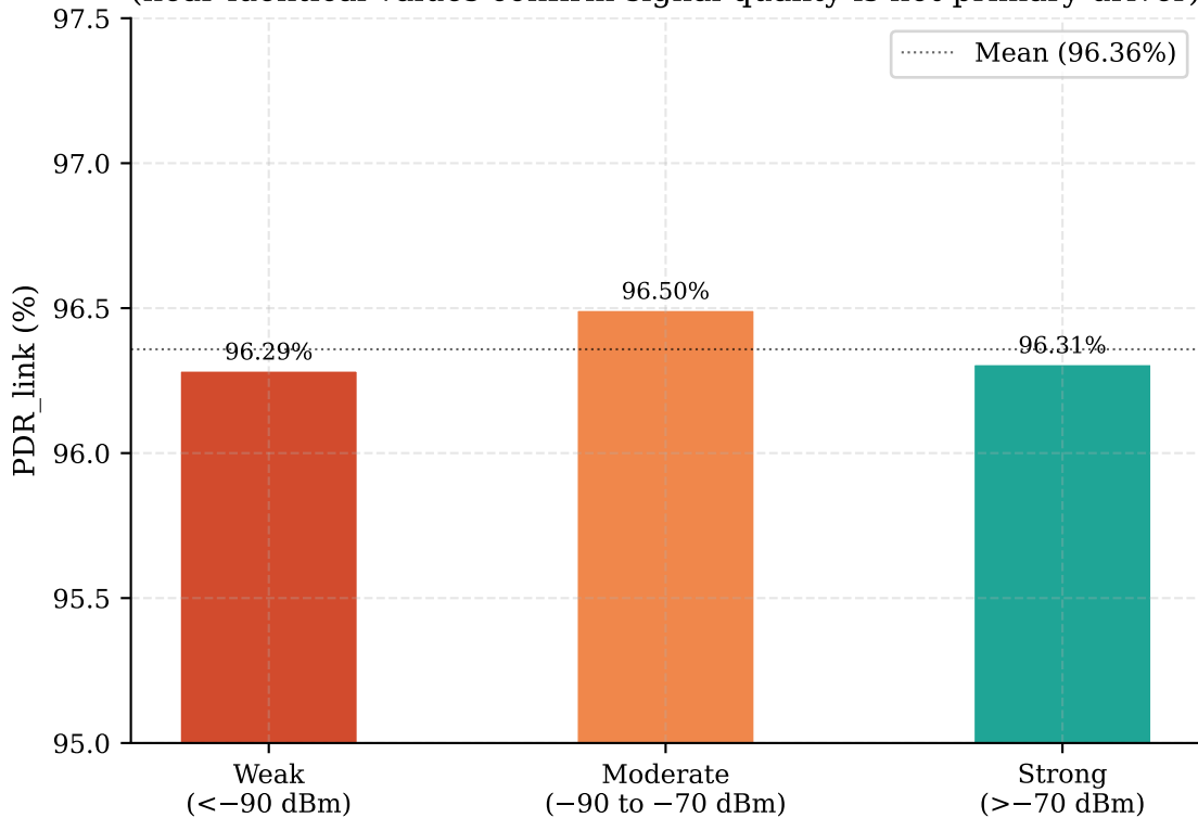
Fig 7.14 — PDR by RSSI Tier (E17) (near-identical values confirm signal quality is not primary driver)
