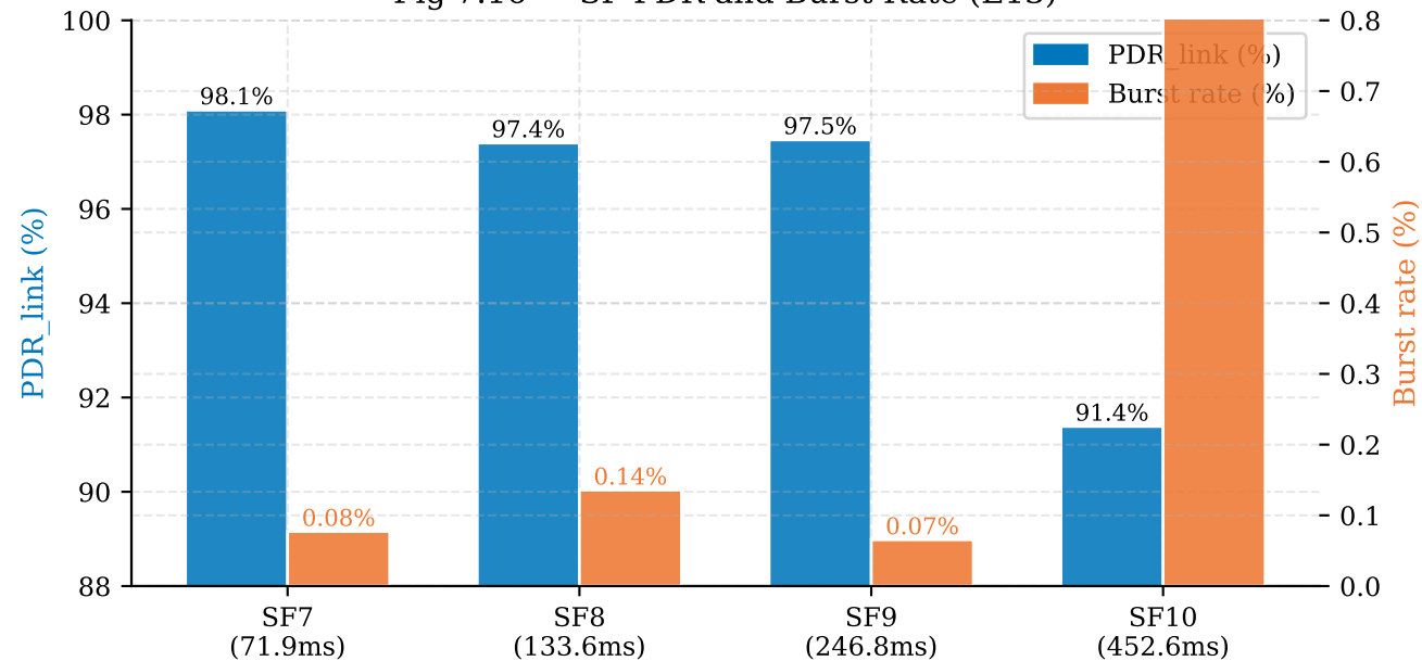
Fig 7.16 — SF PDR and Burst Rate (E13)
