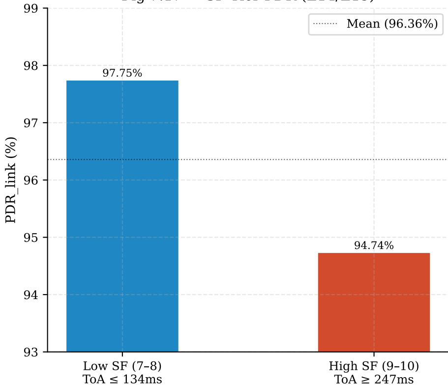
Fig 7.17 — SF Tier PDR (E14/E15)
