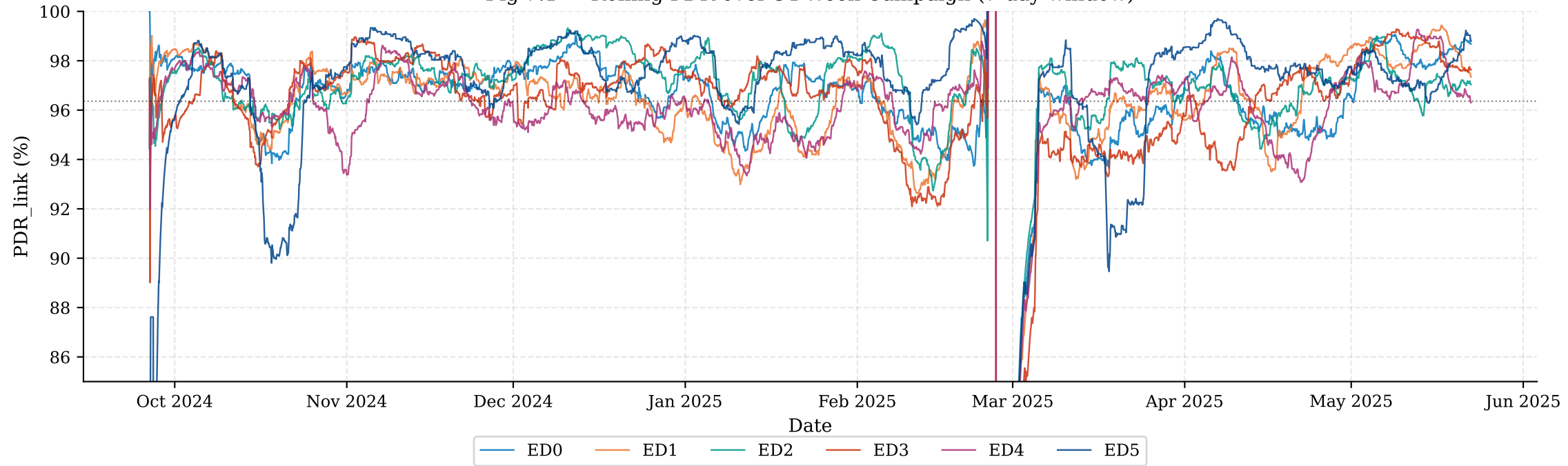
Fig 7.1 — Rolling PDR over 34-Week Campaign (7-day window)
