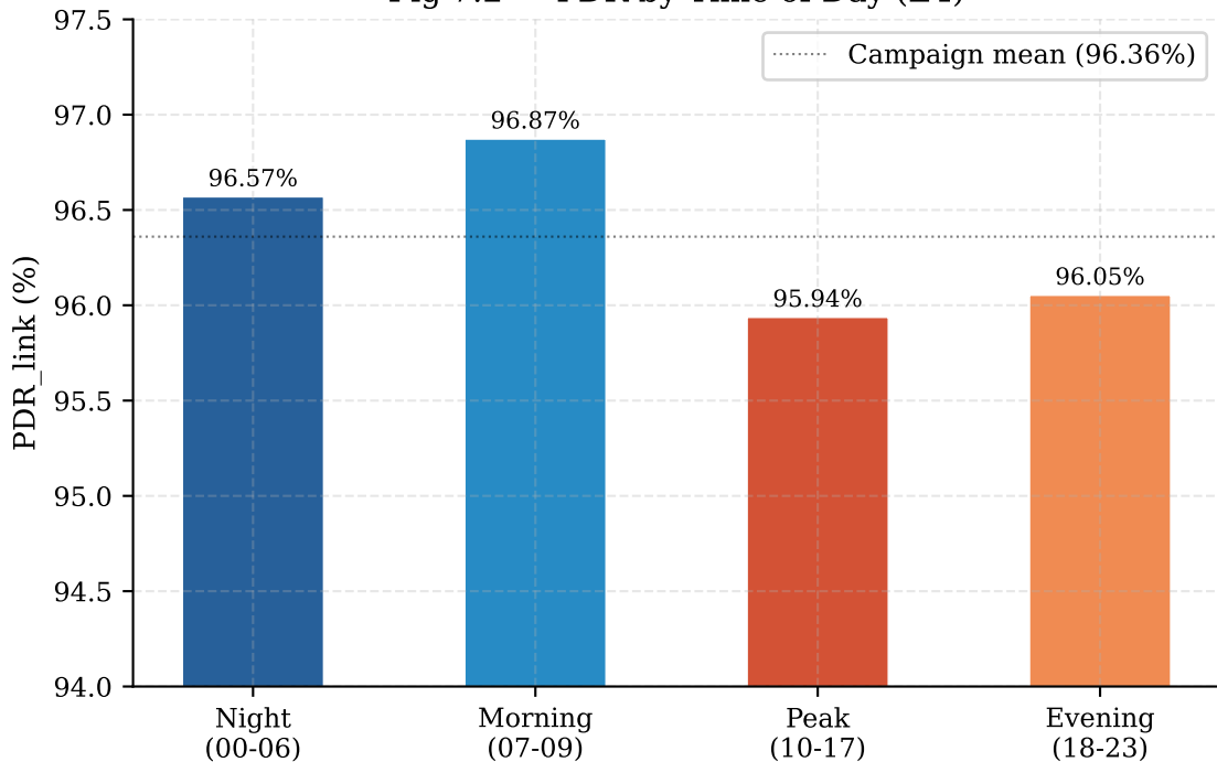
Fig 7.2 — PDR by Time of Day (E4)
