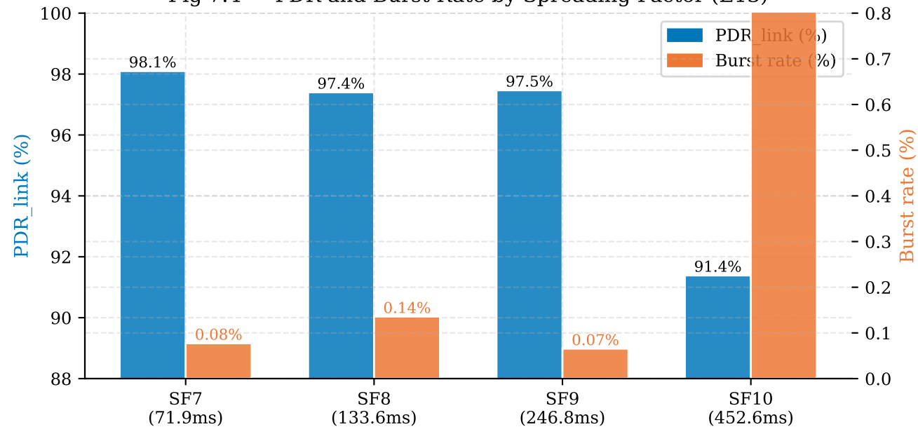
Fig 7.4 — PDR and Burst Rate by Spreading Factor (E13)
