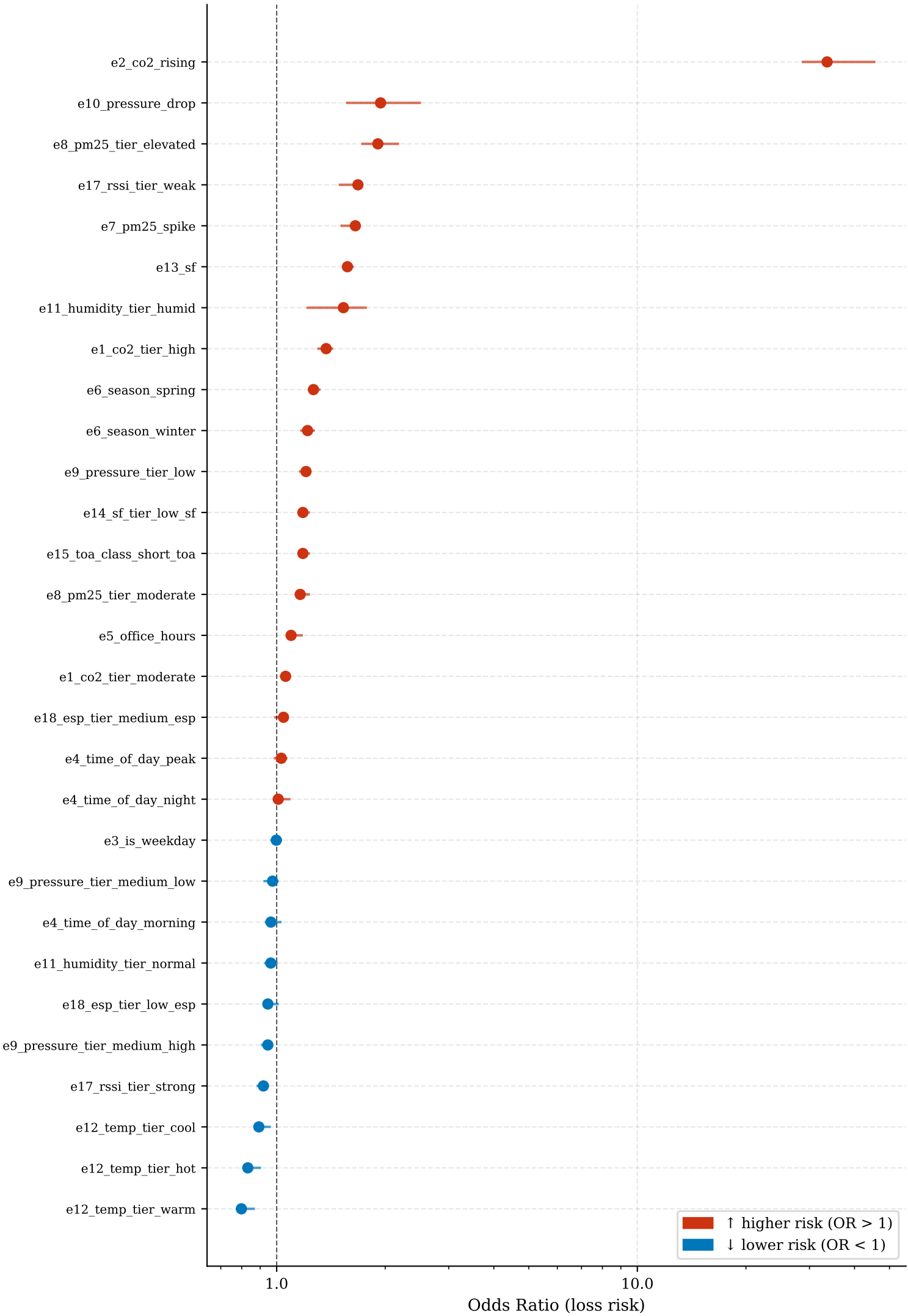
Fig 7.6 — Logistic Regression OR with 95% CI (E1–E18, excl. device effects)
