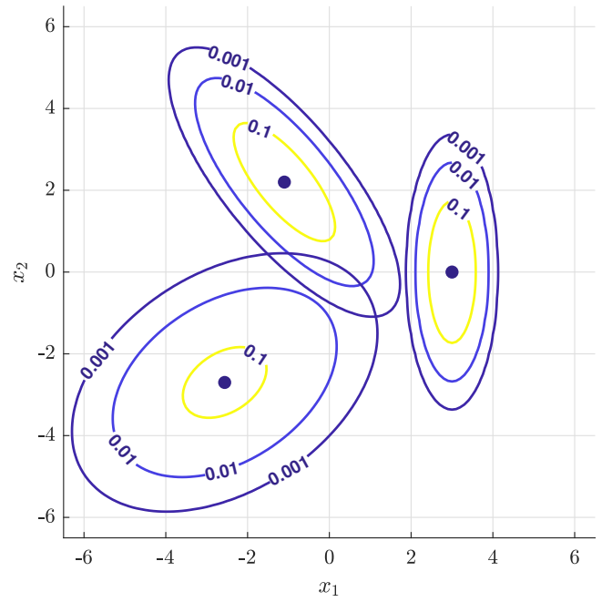
Figure 7: Contour lines of the densities corresponding to the three individual components.
