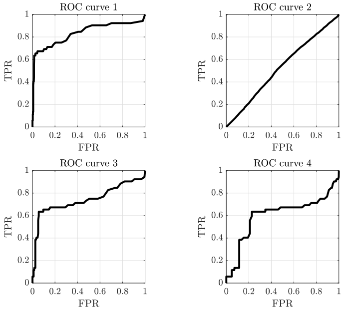
Figure 15: Candidate ROC curves for the classifier.
