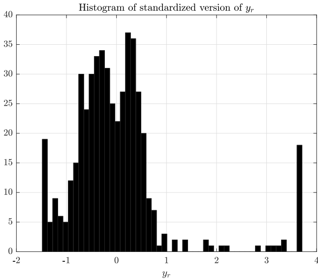
Figure 13: Power consumption y_r (standardized).
