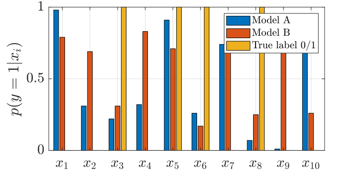
Figure 11: p(y = 1|x_i) for the two models on a test set of 10 points x_1, \dots, x_{10} , and the true labels. If p(y = 1|x_i) > 0.5 , then x_i is classified as Class 1 and otherwise Class 0.
