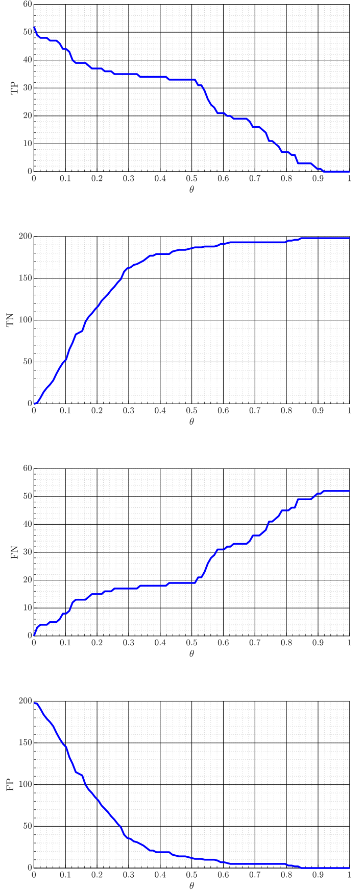
Figure 16: TP, TN, FN, and FP as functions of threshold value \theta .
