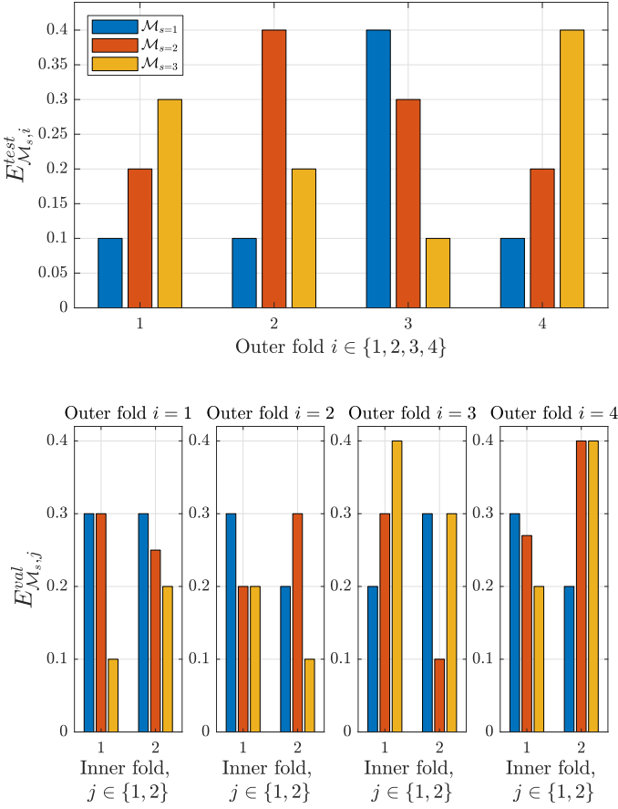
Figure 10: Result of running two-layer cross-validation.
