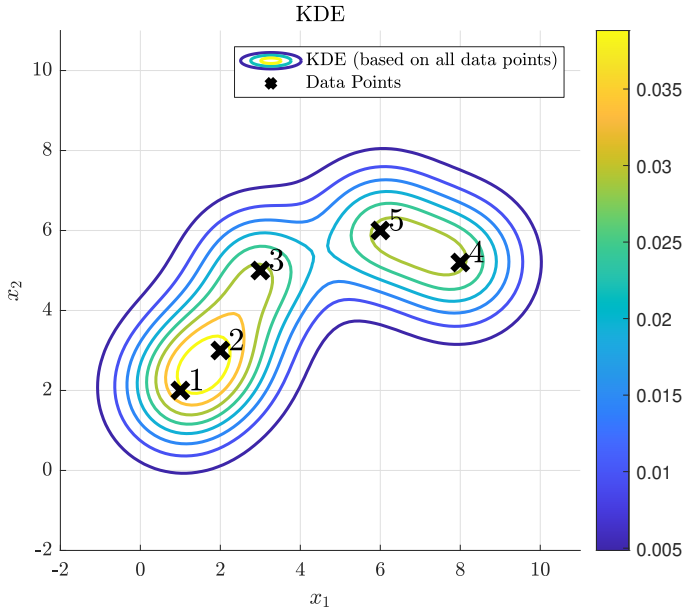
Figure 6: KDE
