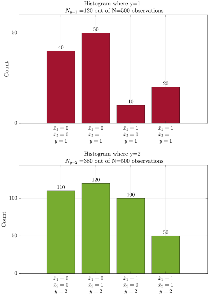
Figure 9: Histogram of a binarized version of the Welding robot dataset described in Table 1.
