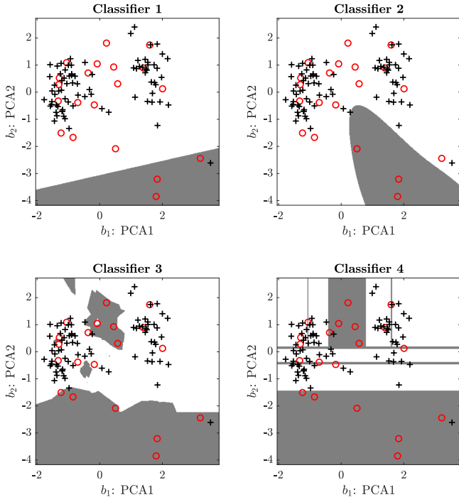
Figure 8: Decision boundaries for four different classifiers trained on the Welding robot dataset when projected onto the first two principal components (only a subset of the observations is shown).
