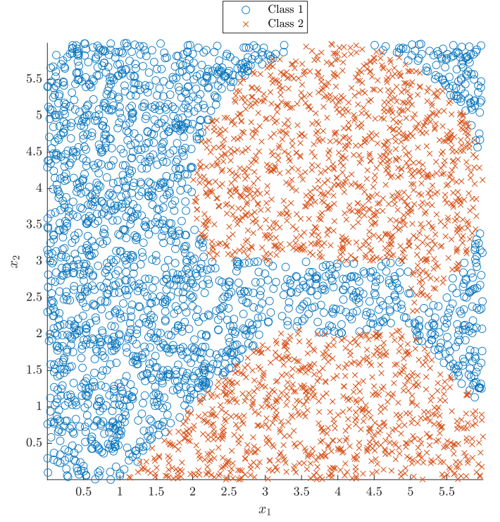
Figure 5: Classification boundary.
