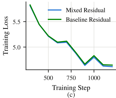
Training Loss at Learning Rate 0.003
