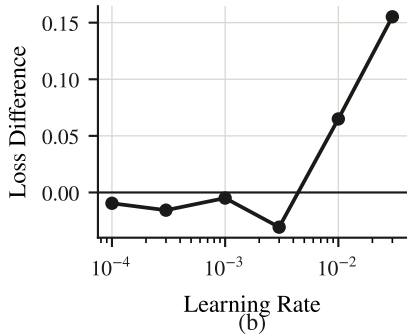
Loss Difference (Mixed - Baseline)
