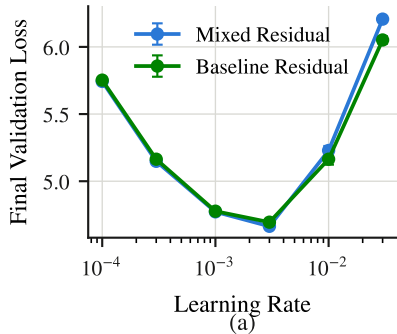
Final Validation Loss vs. Learning Rate
