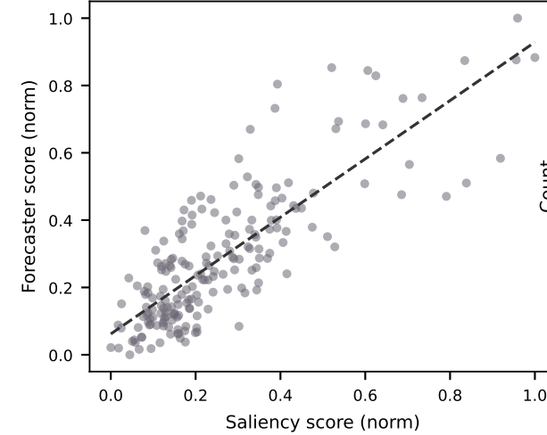
Rank correlation Spearman \rho = 0.774
