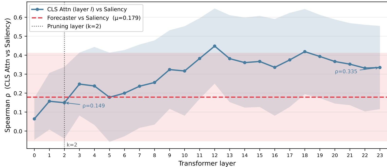
Alignment between CLS attention and Gradient×Input saliency across layers (mean \pm std over 399 correctly classified test images)
