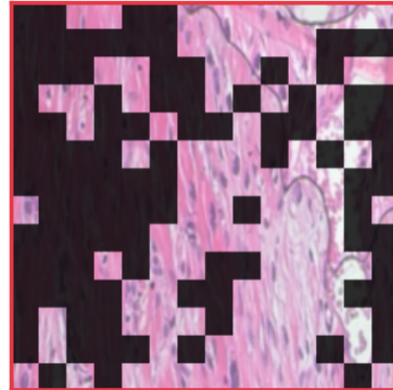
98 / 196 tokens (50%)
