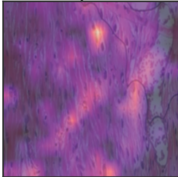
Full sequence
