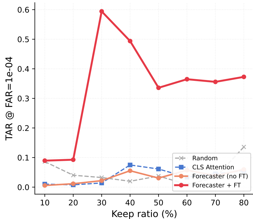
Patch Pruning — BREAKHIS Prune layer: 2
