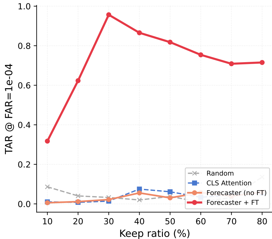
Patch Pruning — BREAKHIS Prune layer: 2
