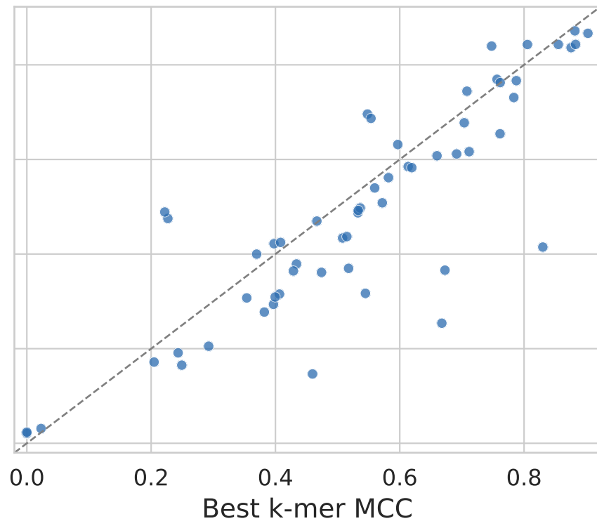
Residual (k=6) vs best k-mer
