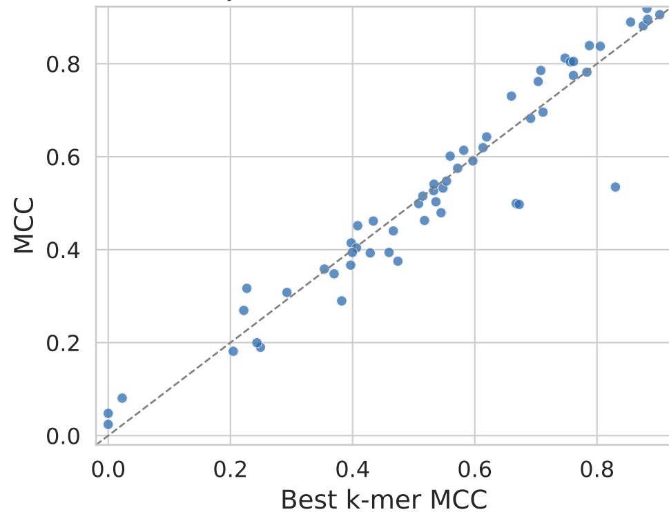
Projection (k=6) vs best k-mer
