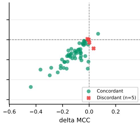
DNABERT-2 (91.2% concordant)
