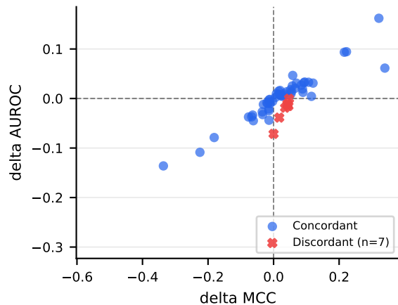
NTv3 (650M) (87.7% concordant)
