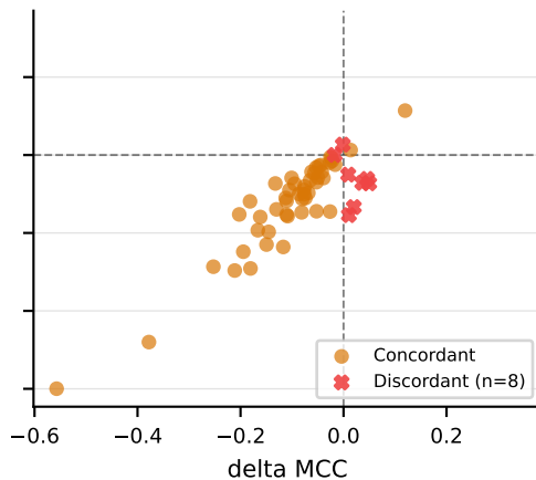
HyenaDNA (86.0% concordant)
