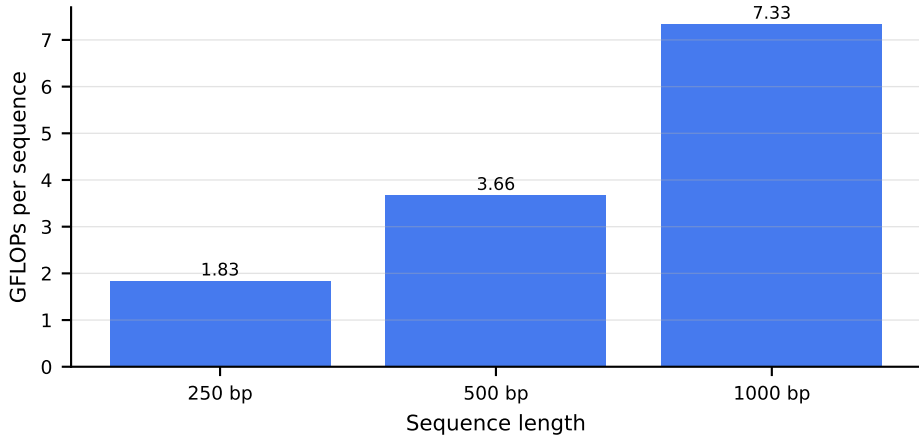
Ablation 7 — NTV3 GPU FLOPs per Sequence (linear scaling with length)
