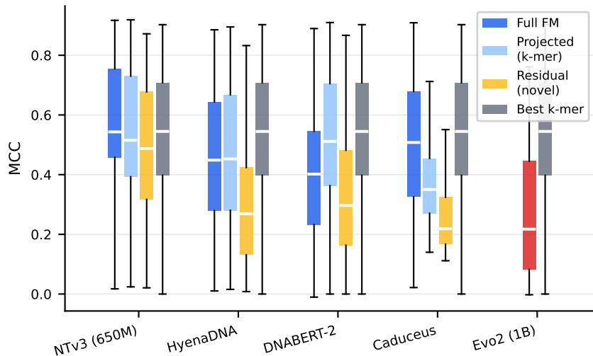
(b) Downstream classification performance
