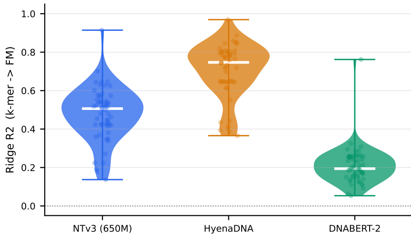
(a) k-mer explainability of FM embeddings (decomposition available for 3 models)
