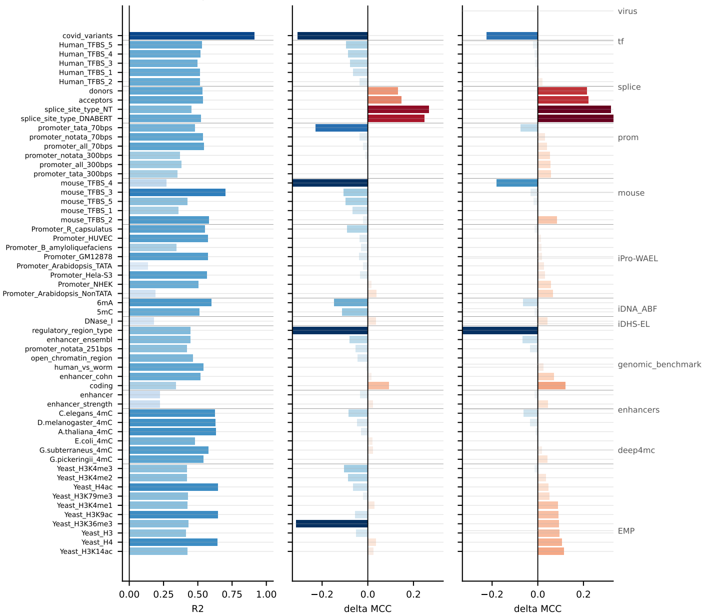
(a) Ridge R2
