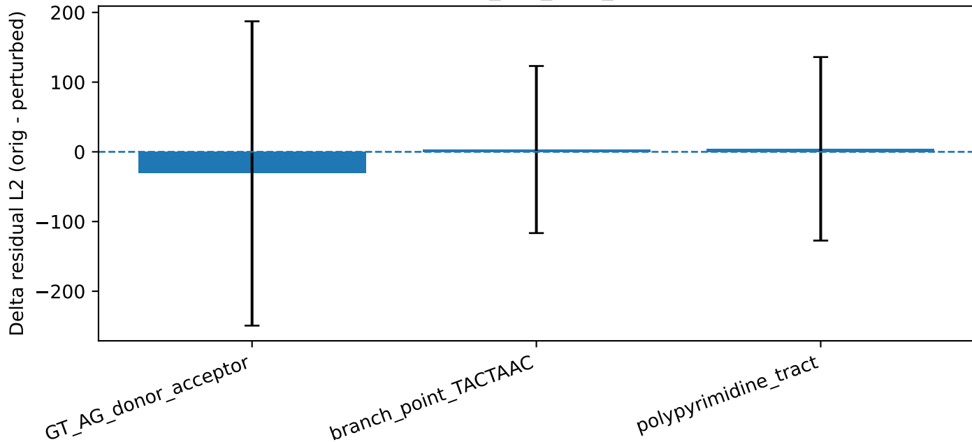
splice/splice_site_type_DNABERT
