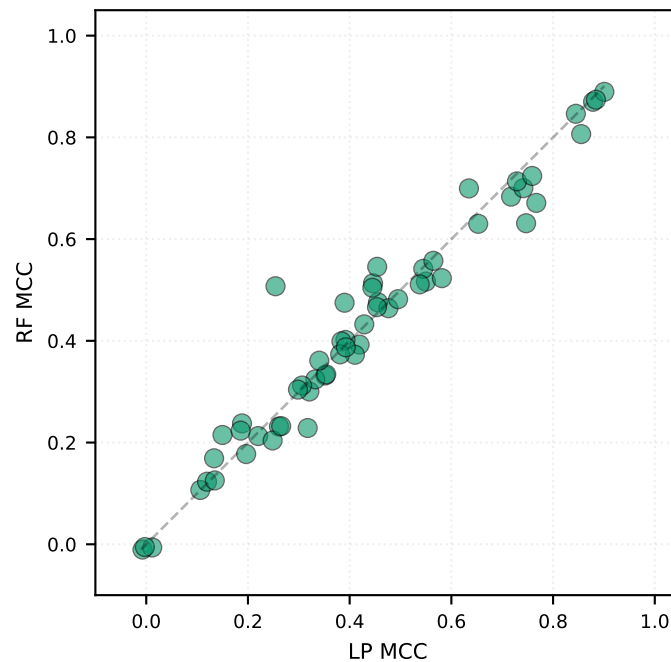
NTv3 (RF wins: 26, LP wins: 31)
