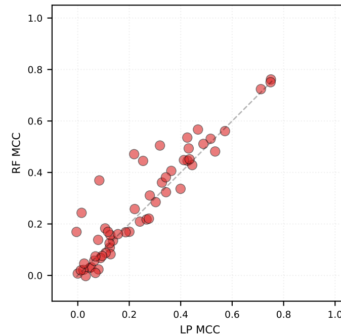
Evo2 (RF wins: 32, LP wins: 24)
