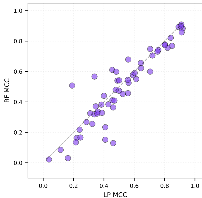
HyenaDNA (RF wins: 7, LP wins: 50)
