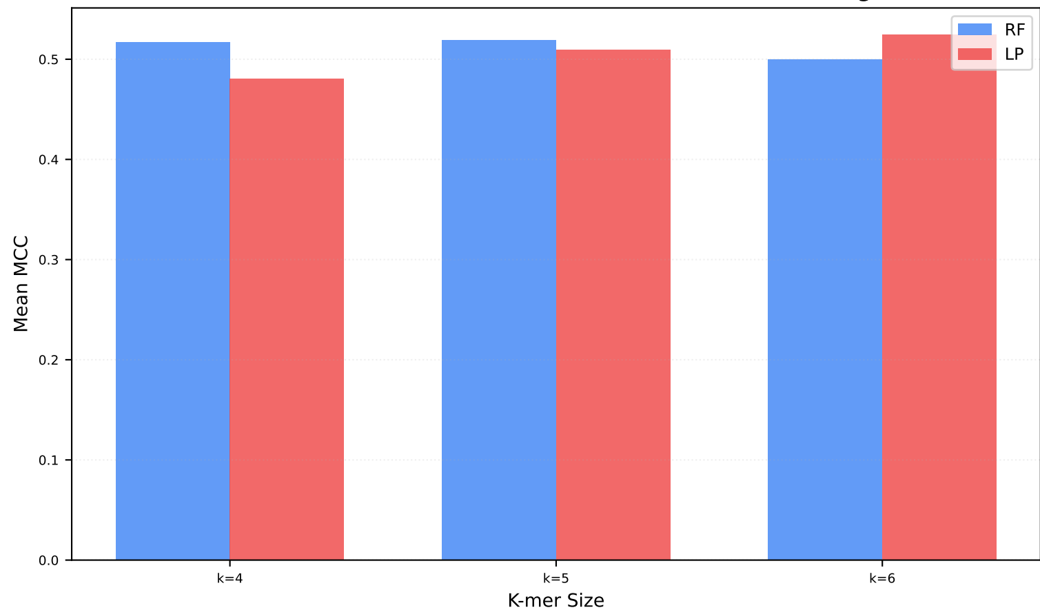
K-mer Classification Performance: RF vs Linear Probing
