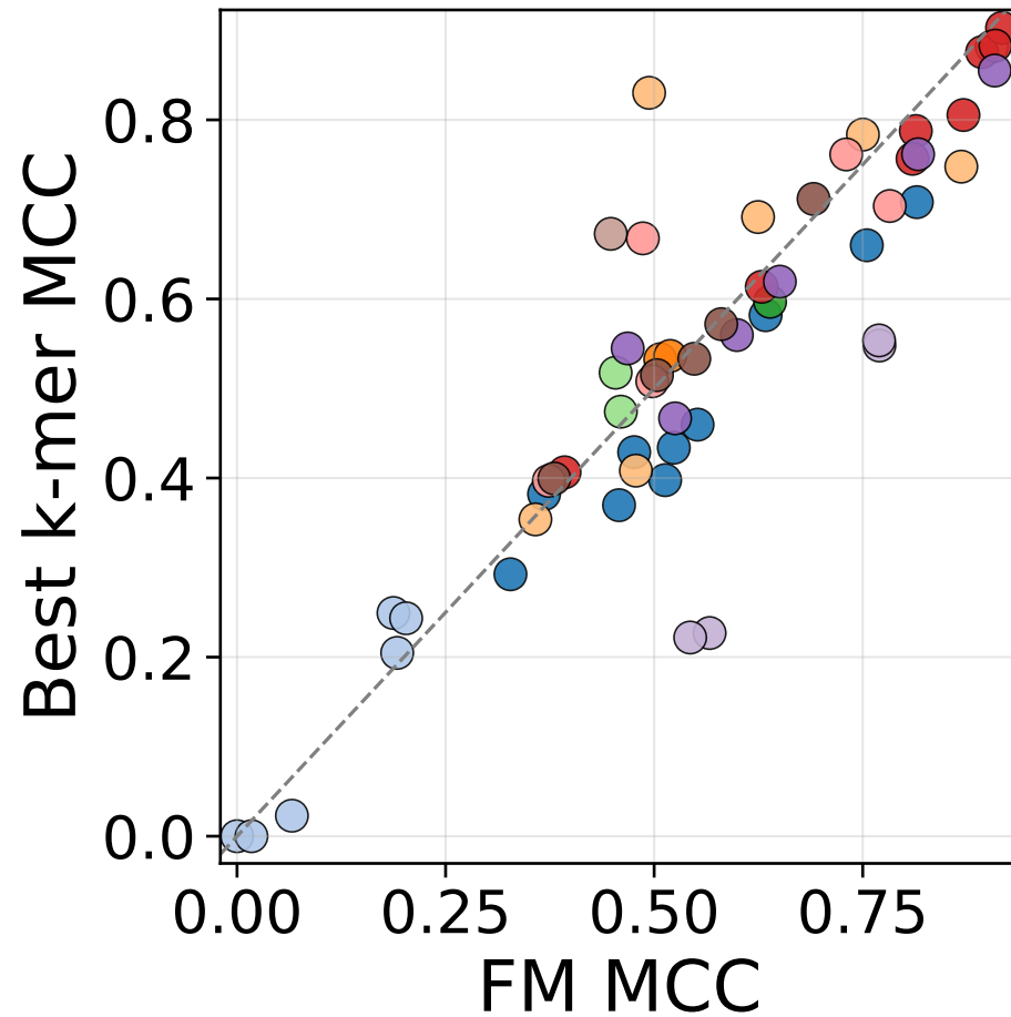
NTv3-650M
