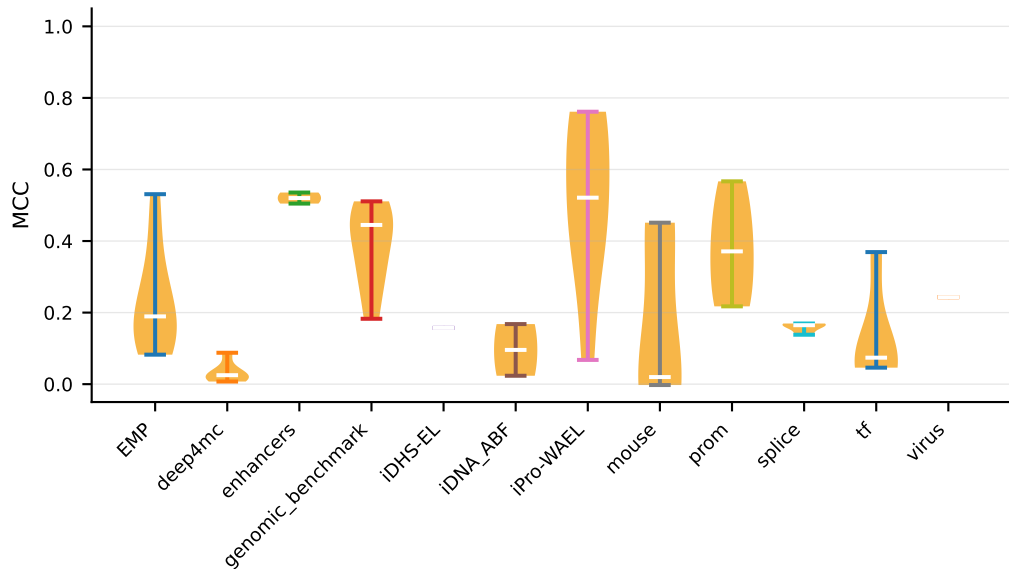
Evo2 (1B) Performance by Dataset Group
