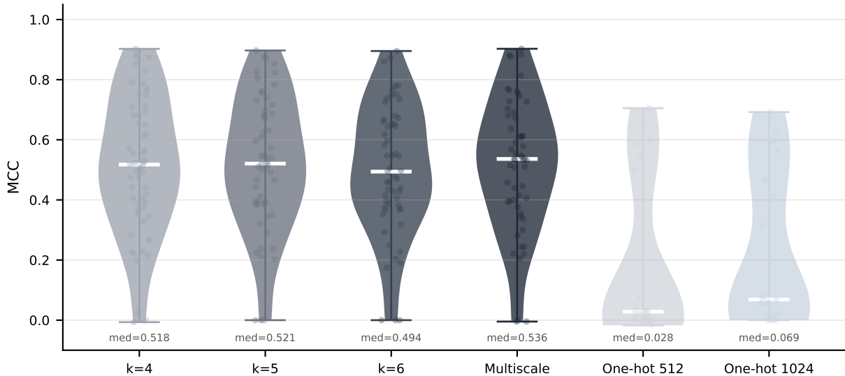
Ablation 1 — k-mer Scale Comparison (57 datasets)
